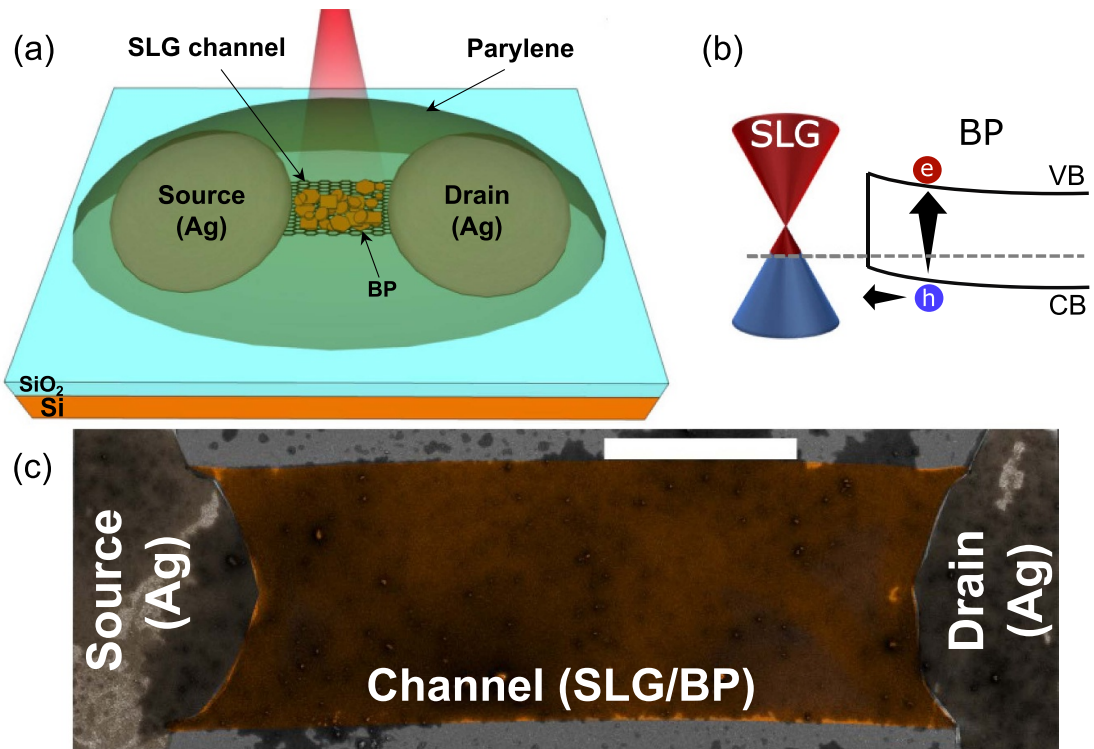
Figure 5. (a) Schematic of SLG/BP PD. SLG is the channel (black honeycomb), BP is the photoactive material (orange), Ag is used for electrodes (silver), Parylene C as encapsulation layer (transparent green), incident light (red). (b) Schematic band diagram of SLG/BP interface, showing the BP CB and VB, generation of e/h pairs and transfer of h from BP to SLG. (c) False colour SEM image of SLG/BP PD on \text{Si/SiO}_2 . BP is inkjet-printed on SLG channel (orange). Ag inkjet-printed source and drains are shown in silver. Scale bar 15\text{ }\mu\text{m} .
