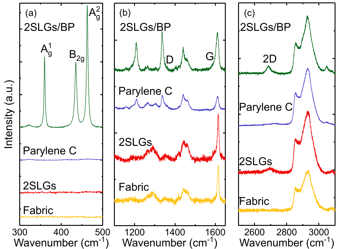
Figure 14. (a), (b), (c) Raman spectra at 514.5 nm of fabric (amber), 2 SLGs on fabric after patterning and PVP removal (red), parylene C on fabric (blue), and 2 SLGs/BP with encapsulation of parylene C (green).
