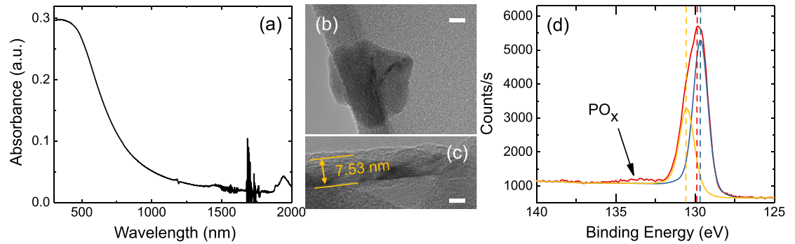
Figure 4. (a) Absorbance of LPE BP. The ambient moisture absorbed by the IPA results in absorbance variations at \sim 1700\text{--}1800\text{ nm} [41]. The dispersions are diluted 6 times to avoid detector saturation. (b) HRTEM image of representative BP flake, scale bar 10 nm. (c) Zoom of (b), scale bar 5 nm. The crystal plane spacing is \sim 0.21\text{ nm} , corresponding to the (002) plane of orthorhombic phosphorus [117]. (d) Representative XPS of LPE BP flake, showing the 2p^{3/2} and 2p^{1/2} \sim 129.7 [64, 118] and 130.5\text{ eV} [64, 118]. Small \text{PO}_x sub-bands are seen \sim 134\text{ eV} [118–120].
