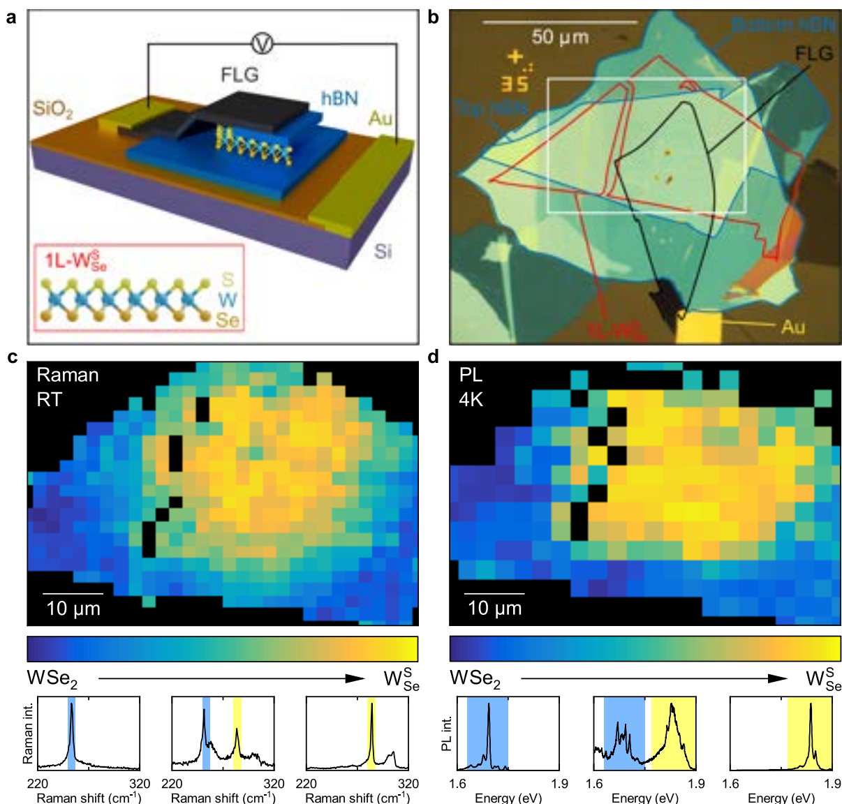
Figure 1. Optical characterization of the Janus 1L- \text{WSe}_2 device. (a) Illustration of the device. Janus 1L- \text{WSe}_2 (inset) is encapsulated in ML-hBN (blue) and electrically contacted by FLG (black). The device is on a n^{+2} Si (purple)/ \text{SiO}_2 (orange) substrate. Au contacts (yellow) allow a voltage to be applied between the FLG and Si. (b) Optical image of the device. 1L- \text{WSe}_2 is outlined in red, the top and bottom ML-hBN in blue, and FLG in black. (c) Raman map of the device, in the region highlighted by the white box in (b), acquired at room temperature using 2.33 eV optical excitation. The color coding shows the relative intensity between the 1L- \text{WSe}_2 E' + A_1' Raman mode ( 254 \text{ cm}^{-1} ), with 100% in blue, and the Janus 1L- \text{WSe}_2 A_1' Raman mode ( 284 \text{ cm}^{-1} ), with 100% in yellow. Regions with no 1L-TMD are shown in black. The arrow indicates conversion from 1L- \text{WSe}_2 to 1L- \text{WSe}_2^S . Raman spectra from unconverted, partially converted, and fully converted locations are shown below the Raman map, with the color shading indicating the Raman modes above. (d) PL map of the device in the region highlighted by the white box in (b), acquired at 4 K using 2.33 eV optical excitation. The color coding shows the relative integrated PL emission intensity between the 1L- \text{WSe}_2 (1.63 to 1.75 eV), with 100% in blue, and Janus 1L- \text{WSe}_2^S (1.77 to 1.91 eV), with 100% in yellow, spectral bands. Regions with no 1L-TMD are shown in black. The arrow indicates conversion from 1L- \text{WSe}_2 to 1L- \text{WSe}_2^S . Representative normalized PL spectra from unconverted, partially converted, and fully converted locations are shown below the PL map, with the color shading indicating the spectral bands above.
